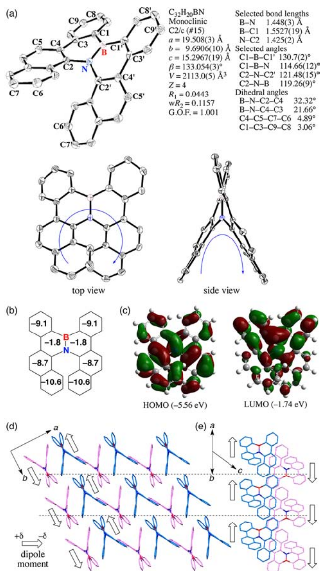
Figure 1. (a) ORTEP drawing and (d, e) packing structure of rac-A obtained by X-ray crystal analysis. Thermal ellipsoids are shown at 50% probability. H atoms have been omitted for clarity. The P enantiomer is shown in blue and the M enantiomer in pink. (b) NICS(1) values and (c) the Kohn–Sham highest occupied MO (HOMO) and lowest unoccupied MO (LUMO) of ( P )- A .
